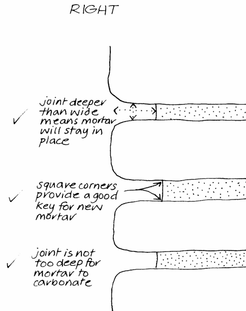
Figure 5. Preparation for Pointing
