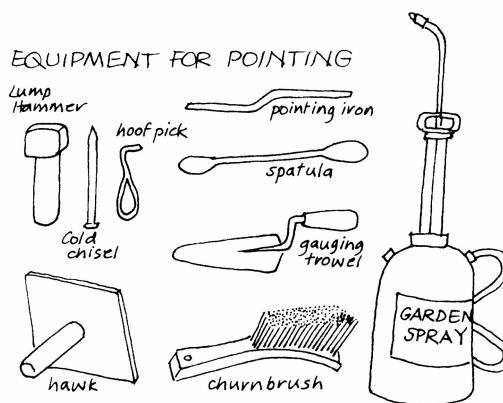
Figure 4 (b) Equipment for Pointing
